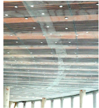
reinforcement for cooling/heating ceilings with dowels type AD
